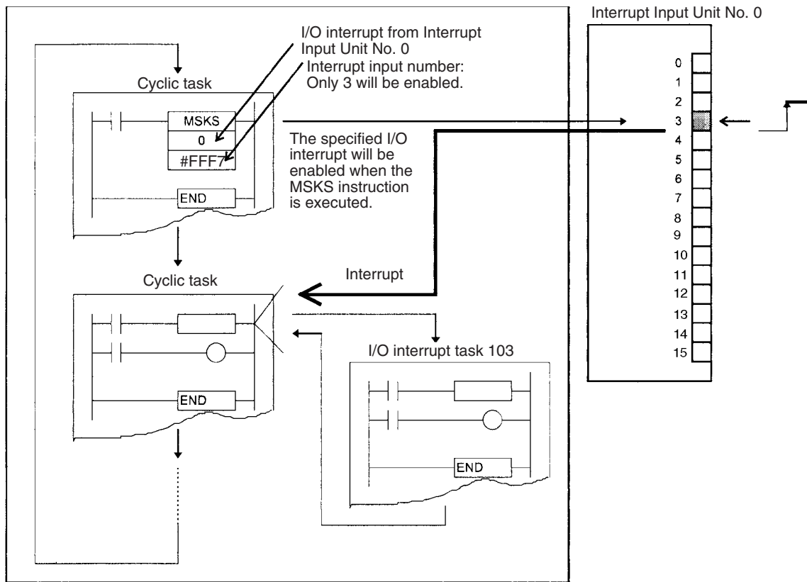
Interrupt Input Unit Numbers, Input Numbers, and I/O Interrupt Task Numbers
