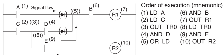
Circuit "a"
