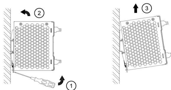
Fig. 2.2 Dismounting
