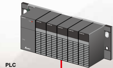
PLC (AH500 Series)
