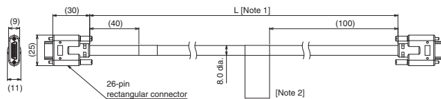
Bend resistant Right-angle Camera Cable FZ-VSLB3
