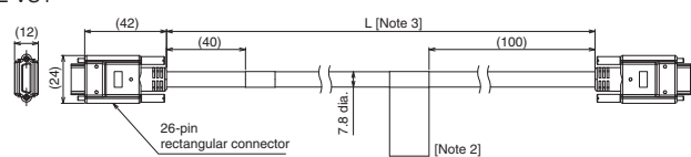
Long-distance Camera Cable FZ-VS4
