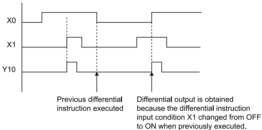
[Timing chart 2]
