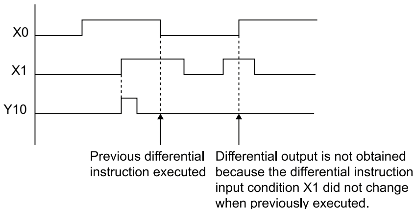
[Timing chart 2]
