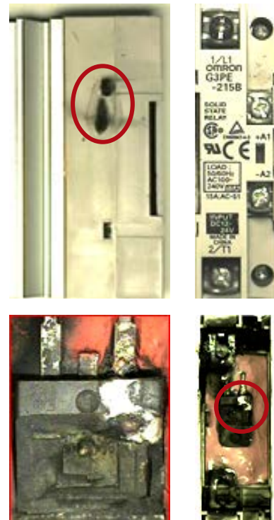
Magnified photograph of a switching element
