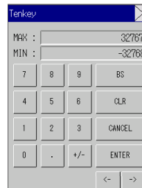
Keypad without Temporary Input
