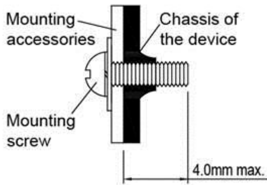
Fig. 4 Mounting Screw
