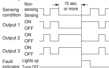
<Timing Chart (In case time-out function works)>
