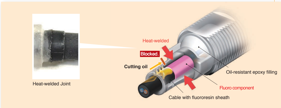
Oil-resistant Proximity Sensors E2ER/E2ERZ
