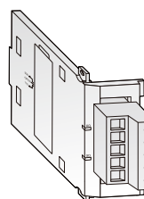
FX3U-485-BD
