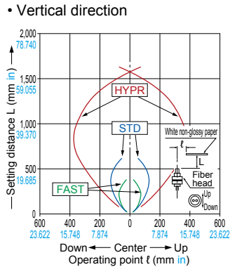
FD-AL11 Reflective type
